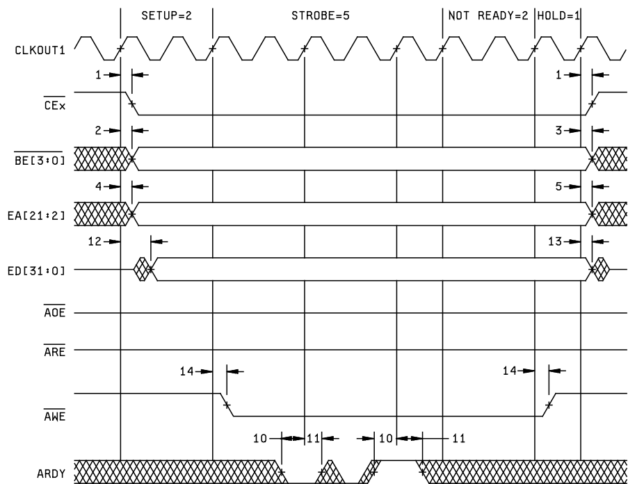
ASYNCHRONOUS MEMORY WRITE TIMING
