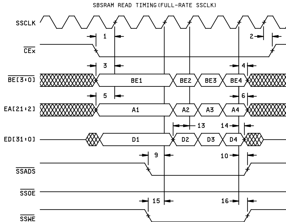
FIGURE 6. Timing waveforms - Continued.
