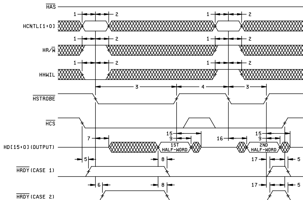
HPI READ TIMING (HAS NOT USED, TIED HIGH)
