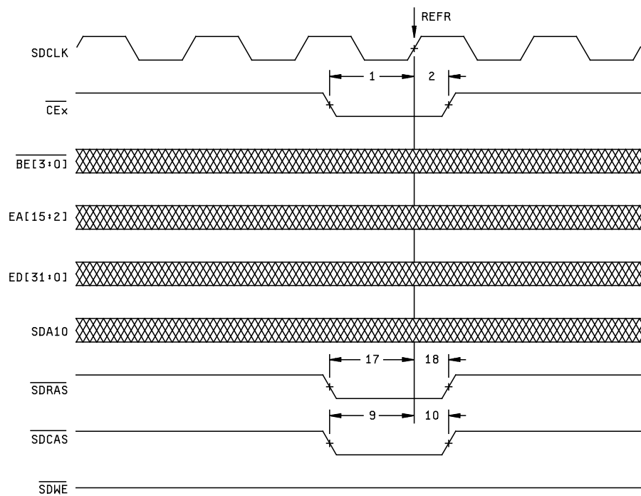
SDRAM REFR COMMAND
