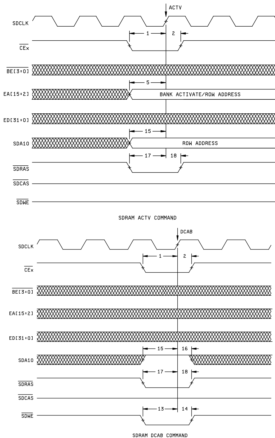
FIGURE 6. Timing waveforms - Continued.
