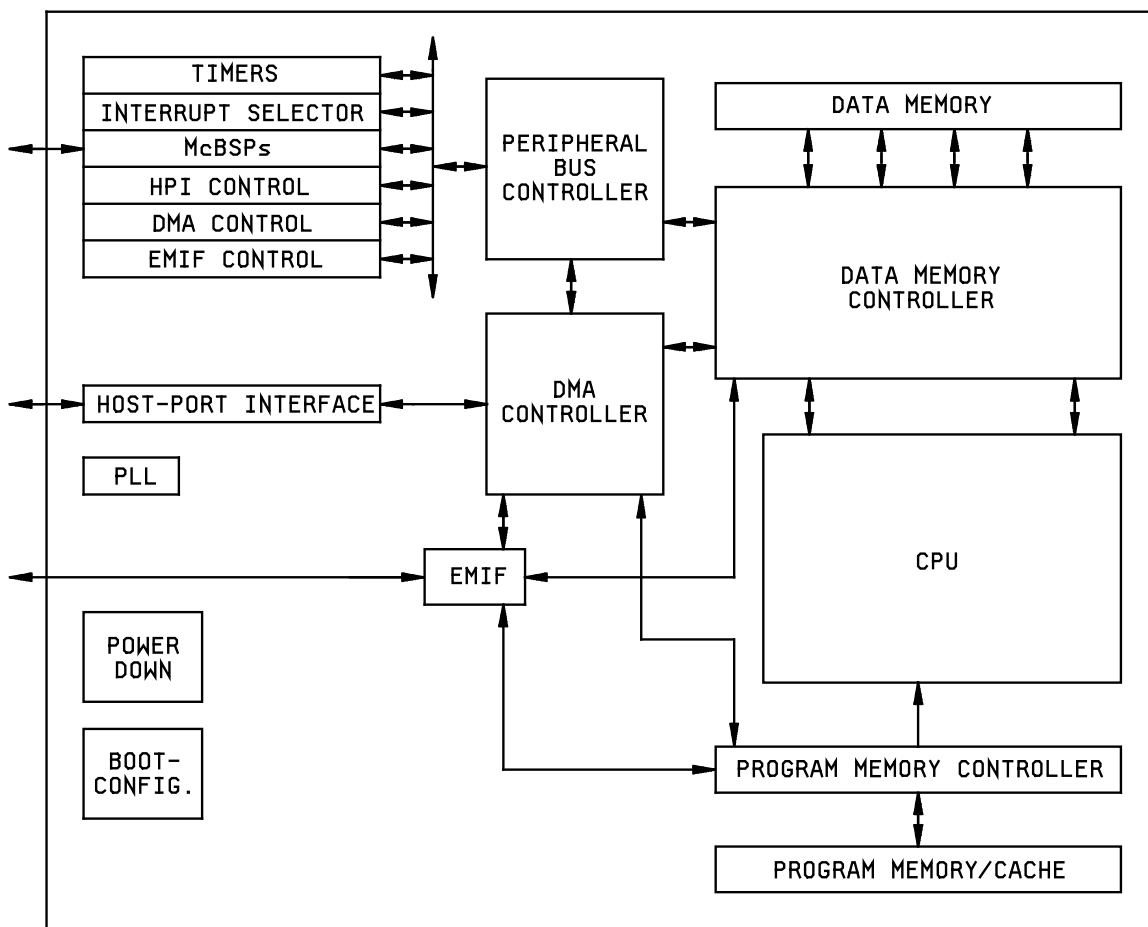
FIGURE 4. Block diagram.
