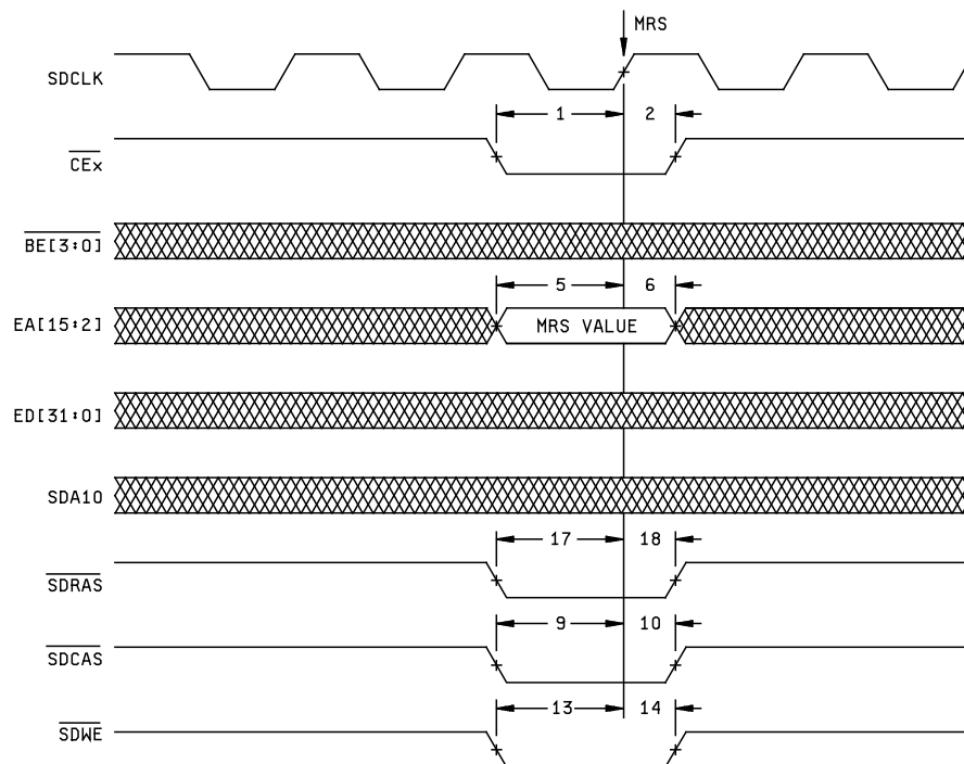
SDRAM MRS COMMAND
